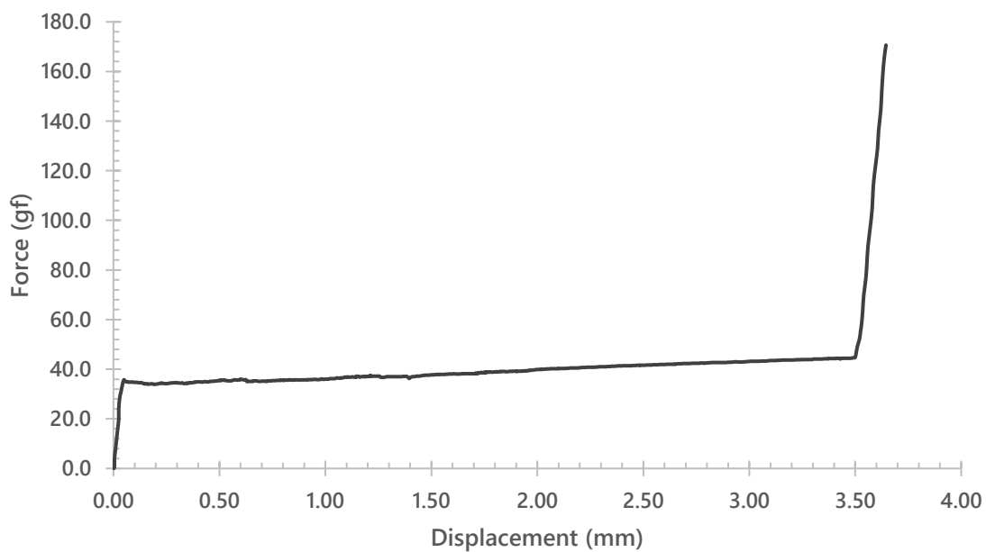
FEKER x Kailh Vanilla Ice Cream Pro (Upstroke)
